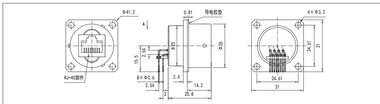
[CT55-8ZW 弯式印制板插座]
